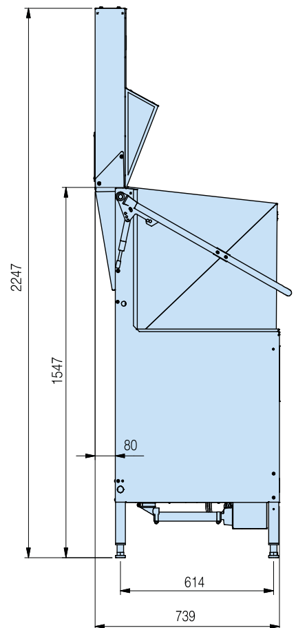
WD-7 GLASS with ECO-FLOW condensing unit and heat exchanger
